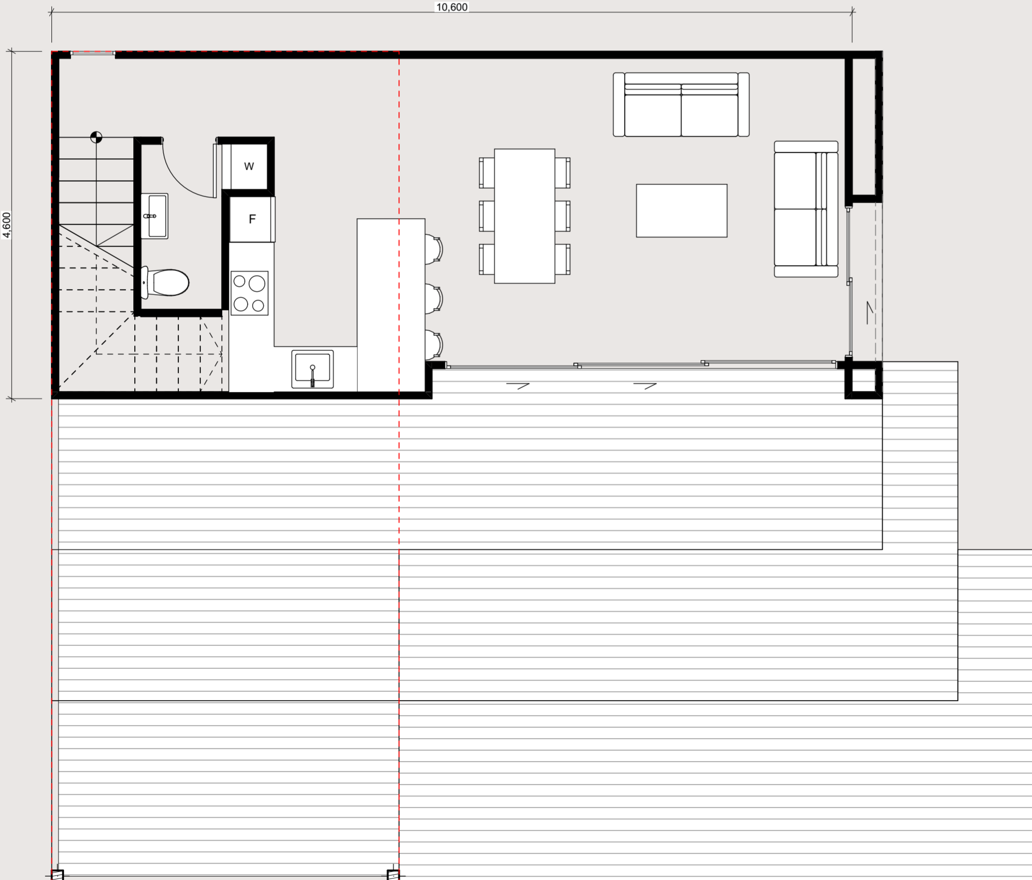
Ground Floor
