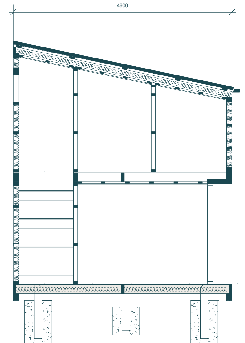
Example Cross Section
