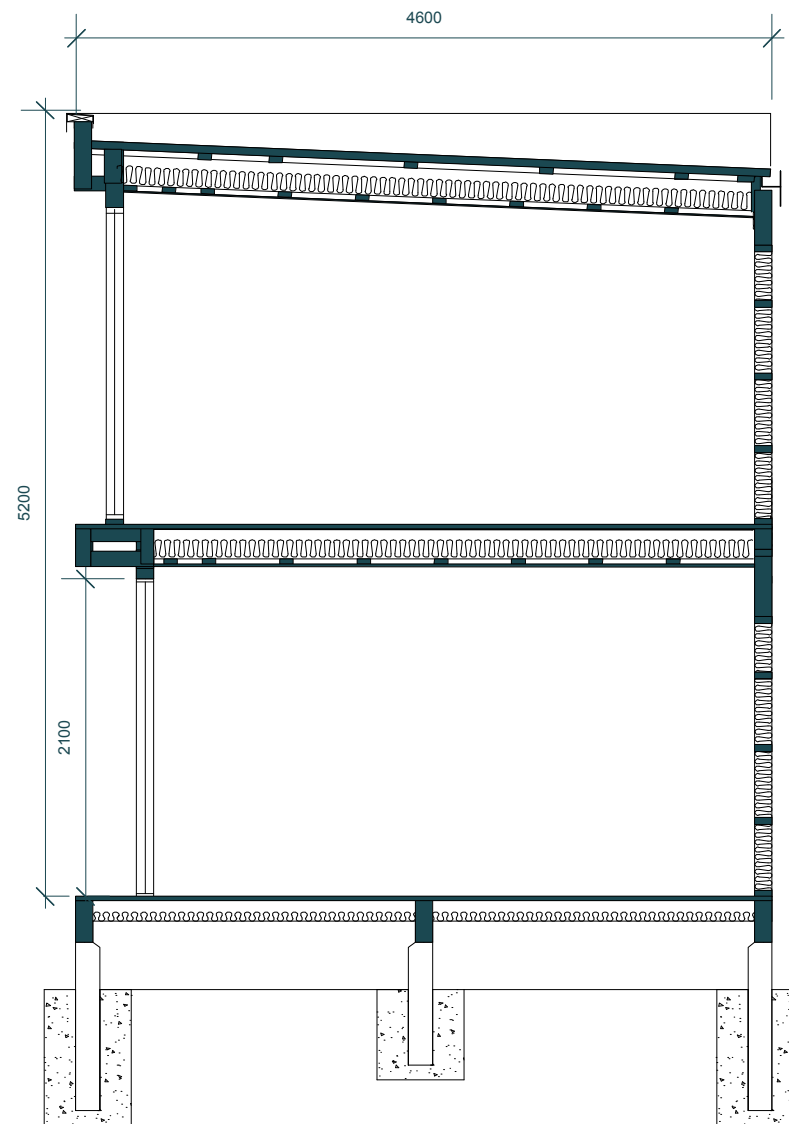
Example Cross Section
